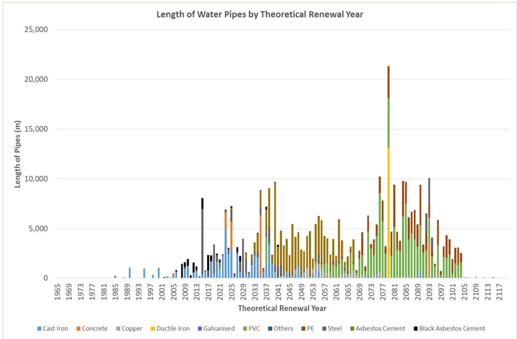
Figure ES-4: Length of Water Pipes by Theoretical Renewal Year
