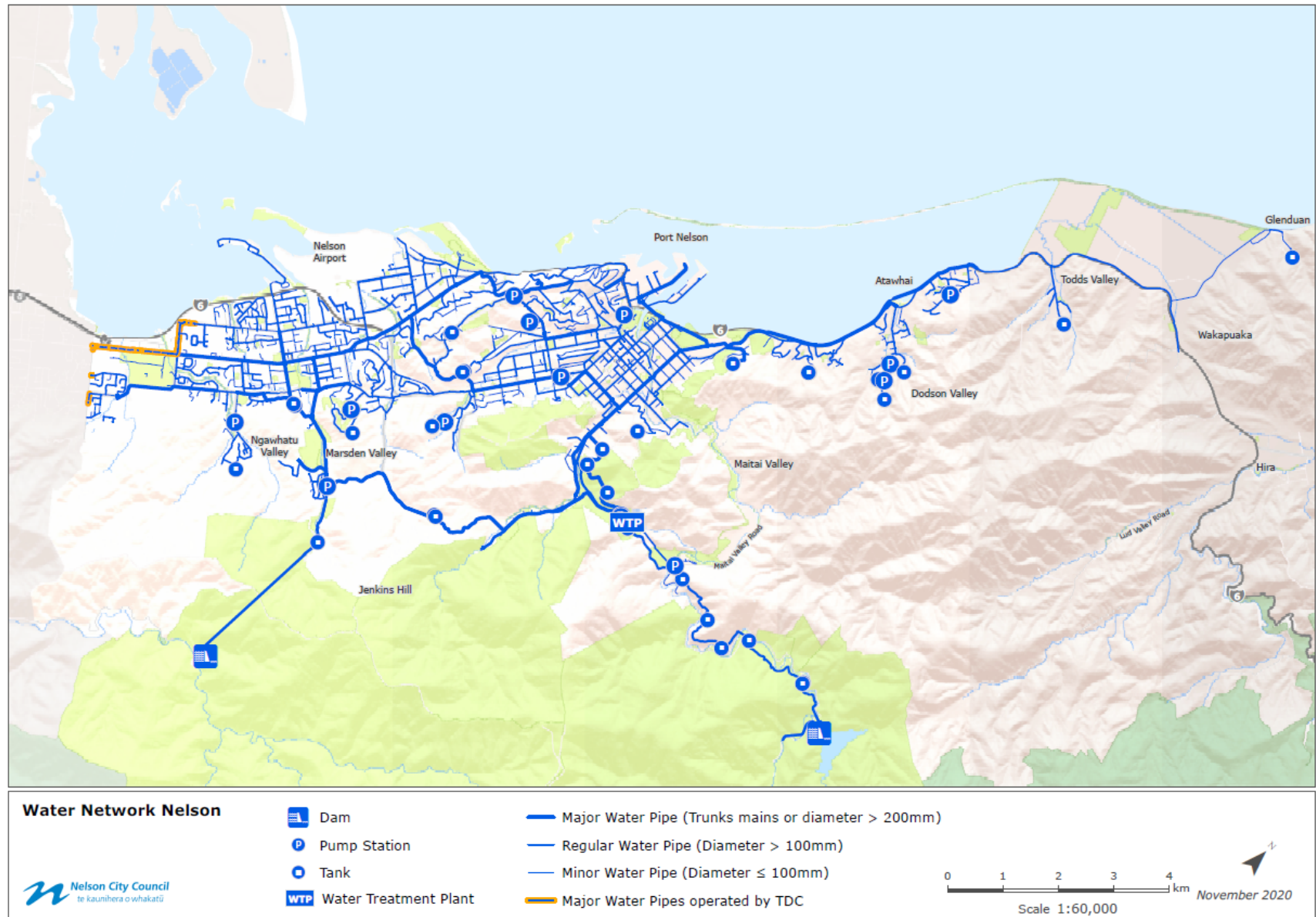
Figure ES-1: Water Network Nelson
