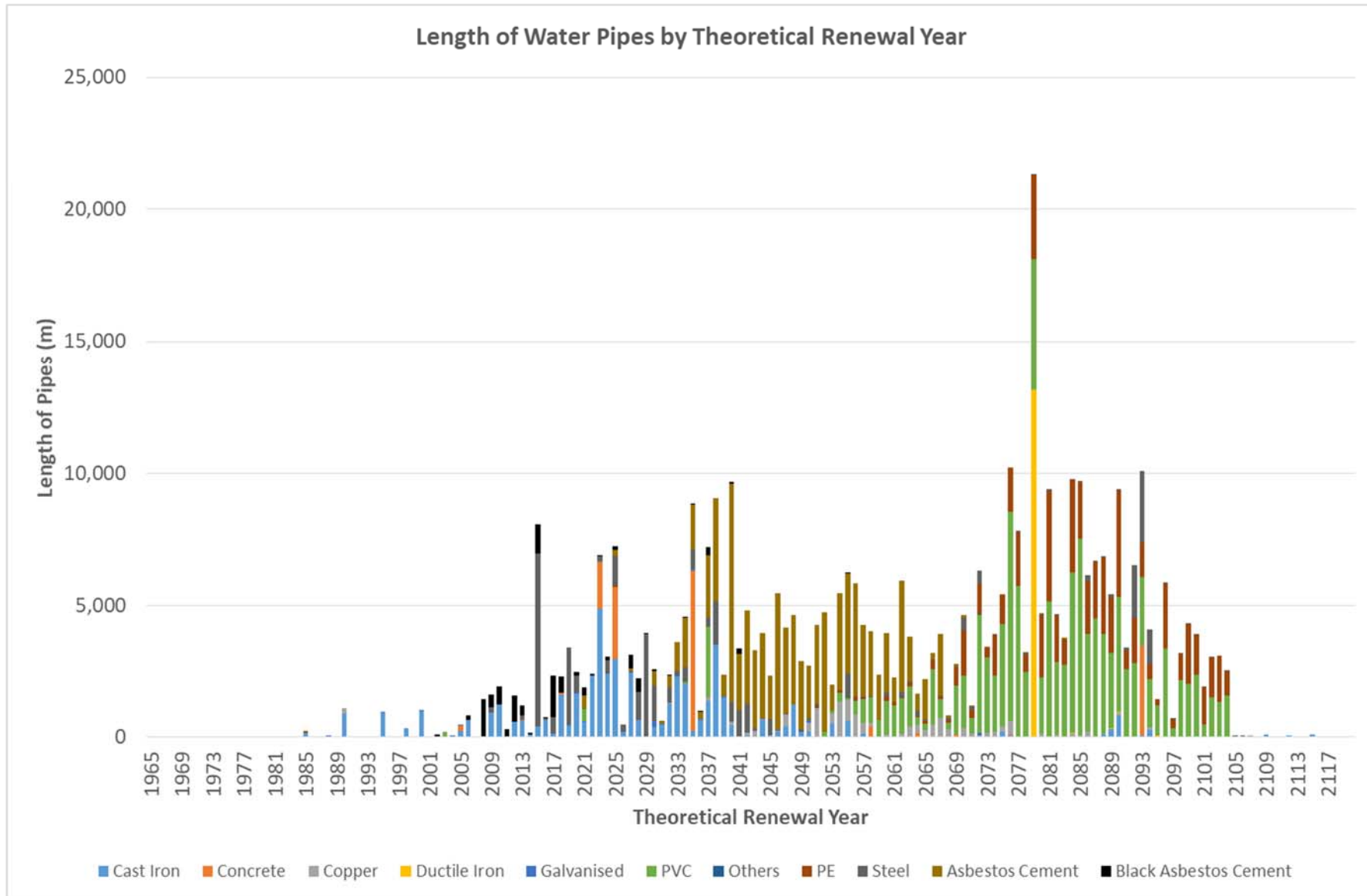
Figure 4-3: Theoretical Renewal Year / Material Distribution
