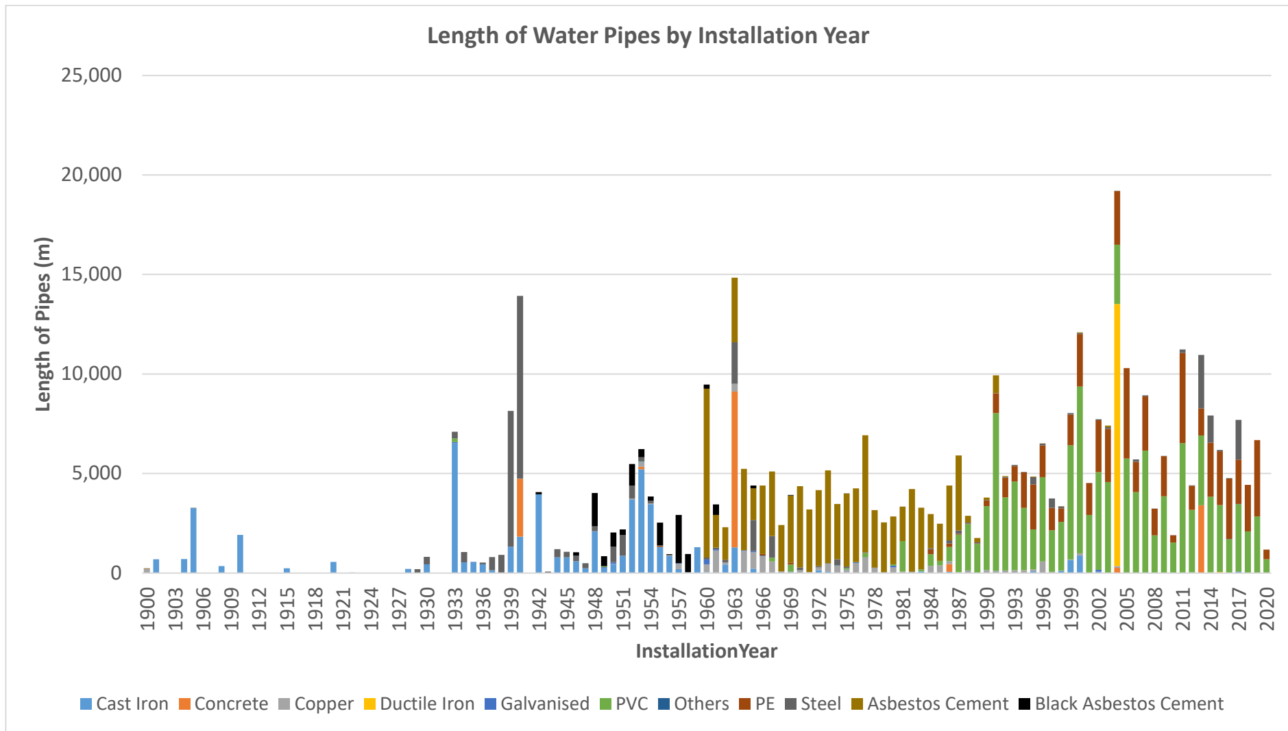
Figure 4-1: Year of Installation / Material Distribution
