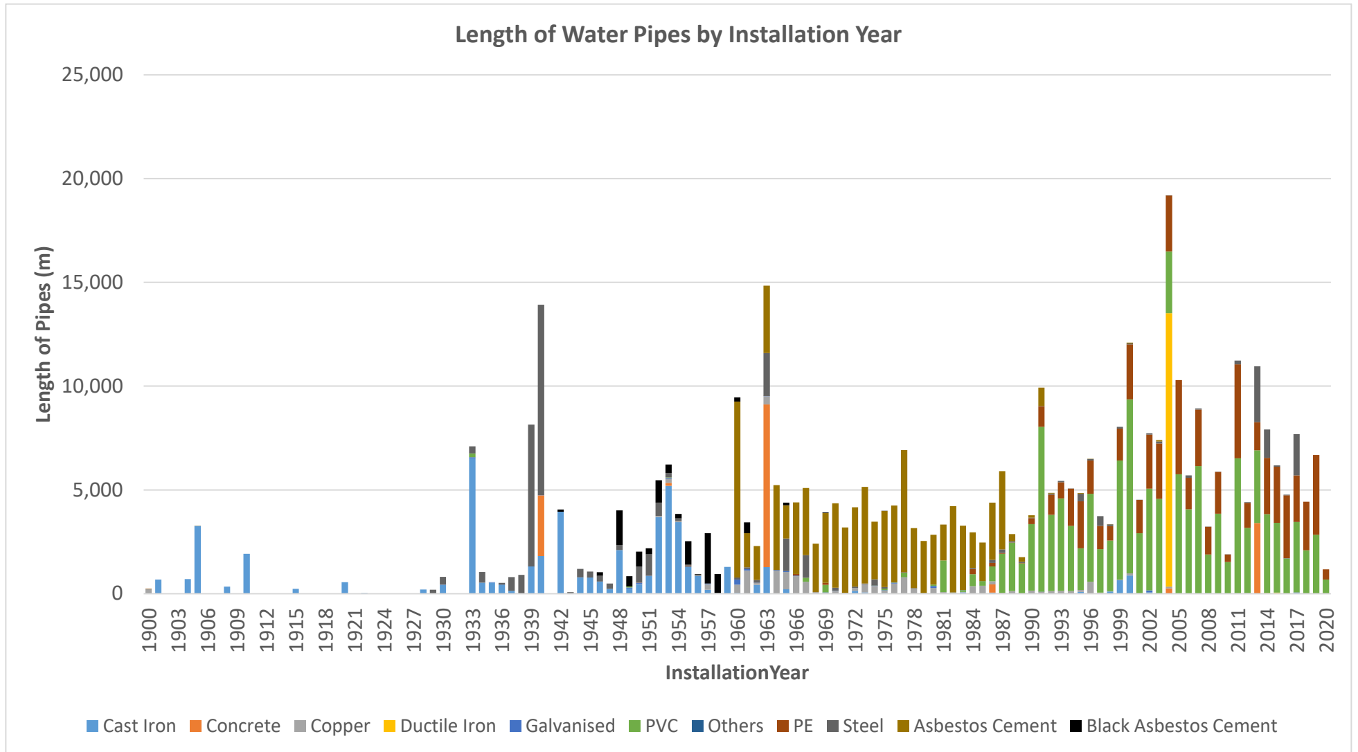
Figure ES-9: Year of Installation / Material Distribution
