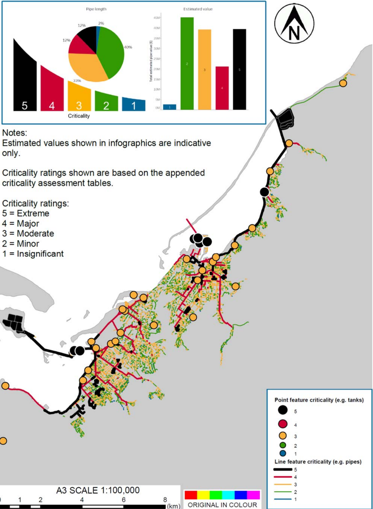
Figure 4-3: Criticality of the components of the wastewater network.
