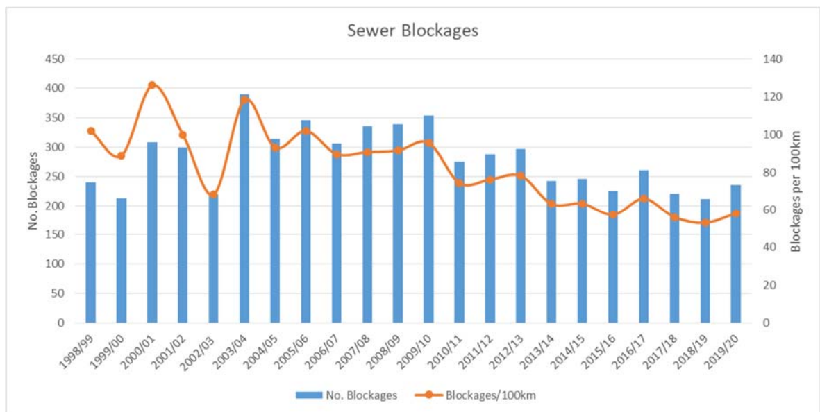
Figure 4-22: Sewer Blockages
