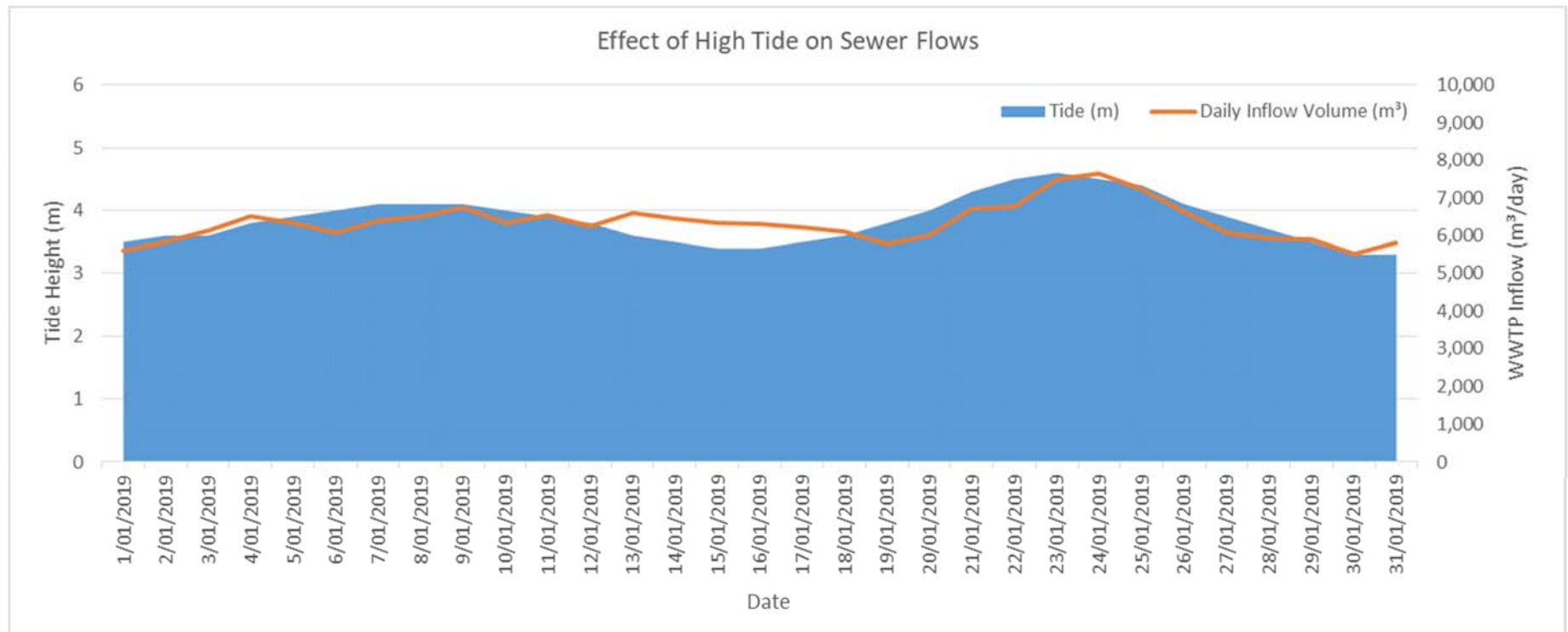
Figure 4-21: Effect of High Tides on Sewer Flows
