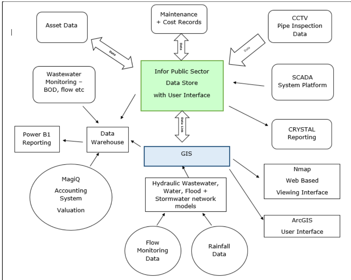
Figure 7-4: Asset Information Systems
