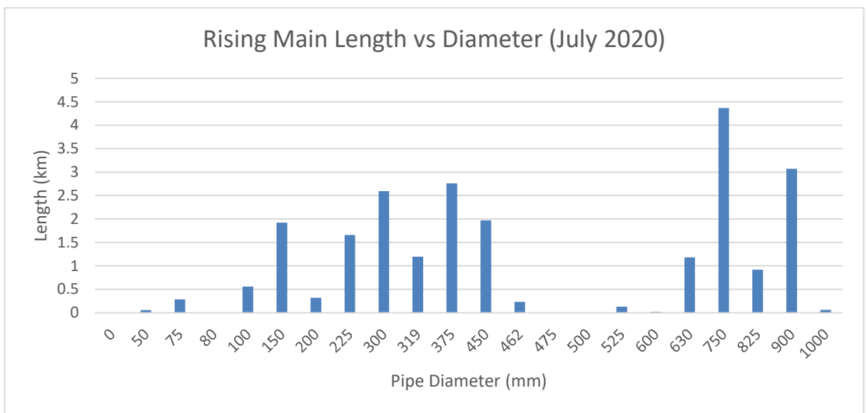
Figure 4-16: Rising main length versus Diameter – 2020
